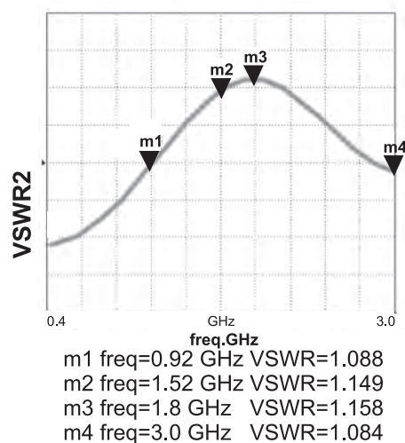
VSWR switched line
