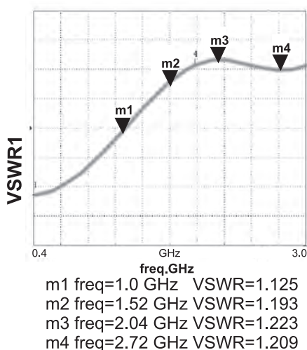
VSWR direct line
